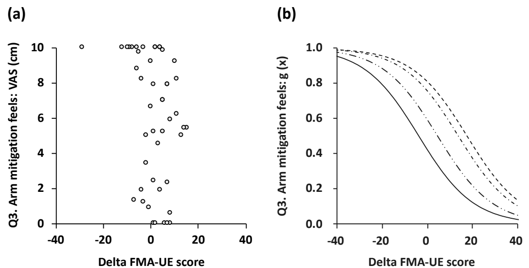
Figure 3. Scatterplots (a) and logistic probability plots (b) showing the association between subjective level of agreement for item 3 and delta FMA score. The logistic curve that discriminated 1 point (strongly disagree with the question) from 2 points (disagree with the question; dashed line), 2 points from 3 points (neither agree nor disagree; dot-dash line), 3 points from 4 points (agree; two-dot chain line), and 4 points from 5 points (strongly agree; solid line) was in a stepwise fashion fit ( p = 0.004 ). FMA: Fugl–Meyer assessment.
